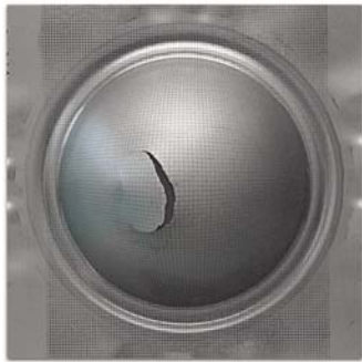
Bulge-Test
