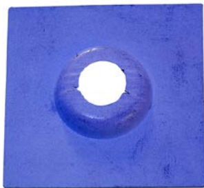
Bore Expanding Test
